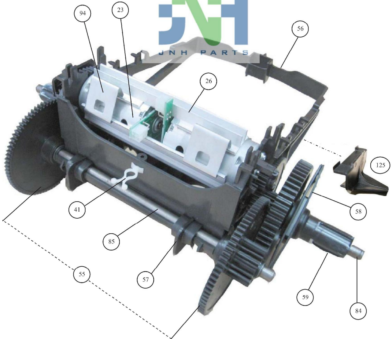
Figure 1.11 SPP0004E Gear Case
