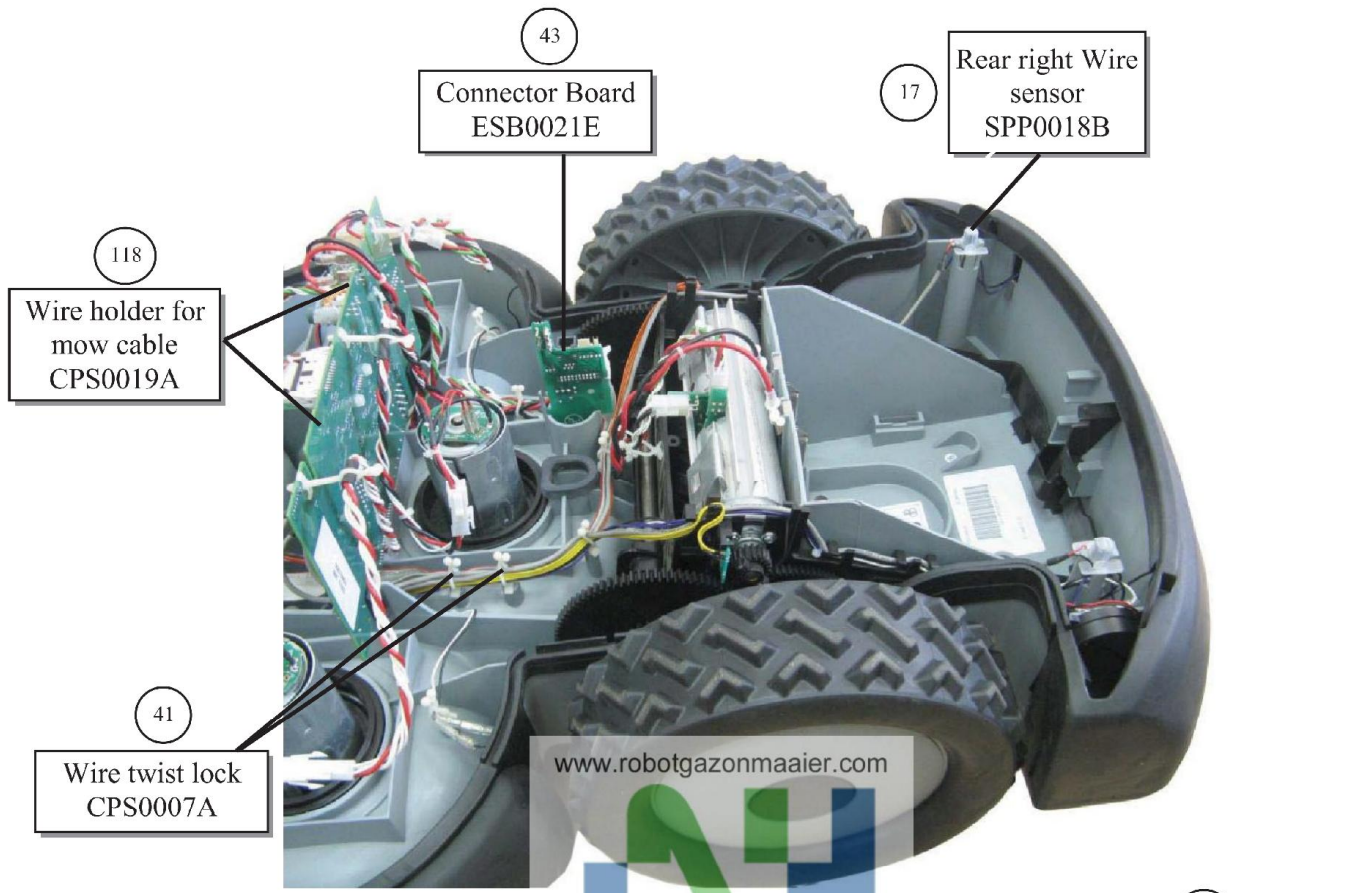
Figure 1.5 Internal view (side)
