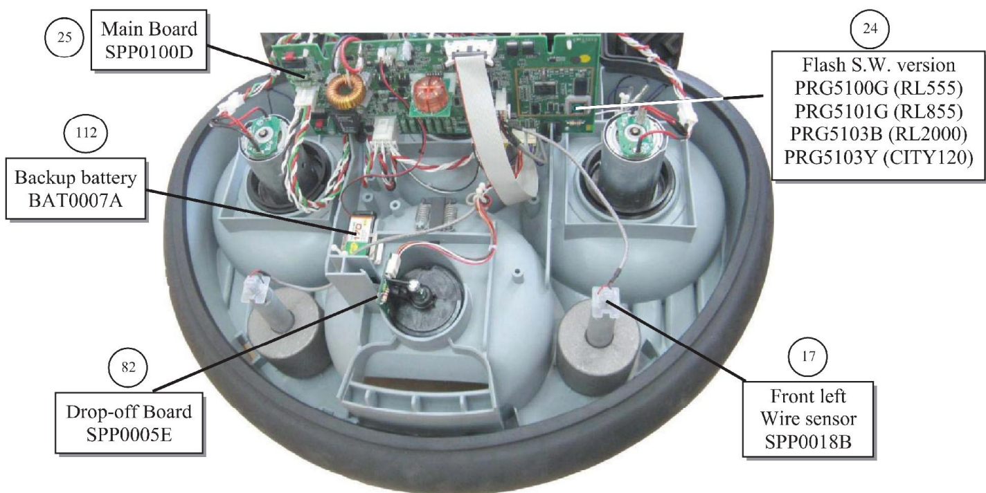
Figure 1.4 - Internal view (front)
